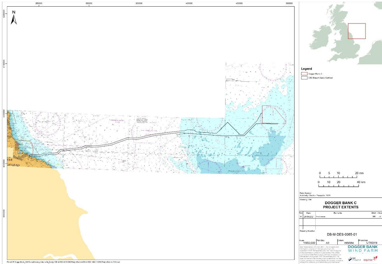
Fig 1 Location Chart DBC Export cable corridor route
